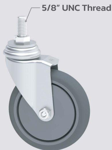
Thread Fitting
