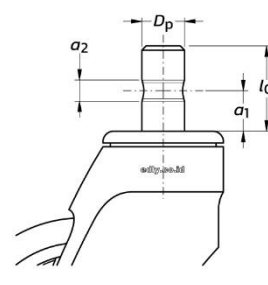
Drawing applicable to castors with Solid Stem Fitting (SF20 or SF32 suffix)
