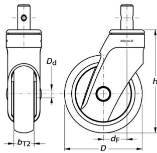
TPRJ Swivel Castors
