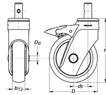
TPRJB Swivel Castors with Total Brake
