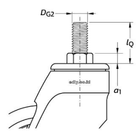
Drawing applicable to castors with Single Bolt Fixing (BF58, BF12, or BFM12 suffix)
