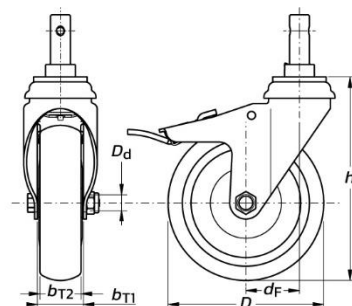
TPRJB Swivel Castors with Total Brake
