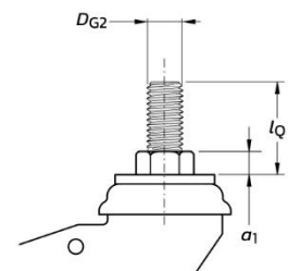
Drawing applicable to castors with Single Bolt Fixing (BF58 suffix)
