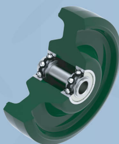
Polyurethane wheel with double precision ball bearings
