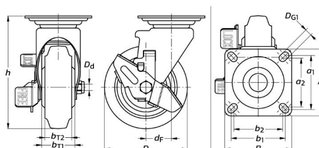
PJ Swivel Castors (applicable to castor frames with or without wheel brake)
