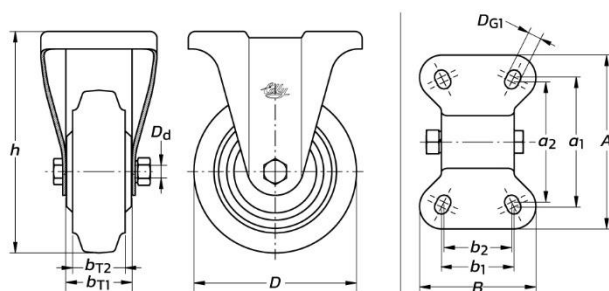
PK Fixed Castors
