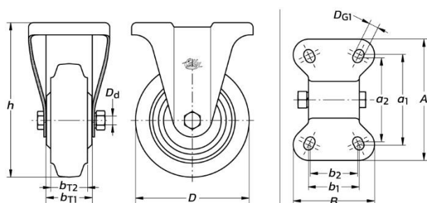
NBK Fixed Castors
