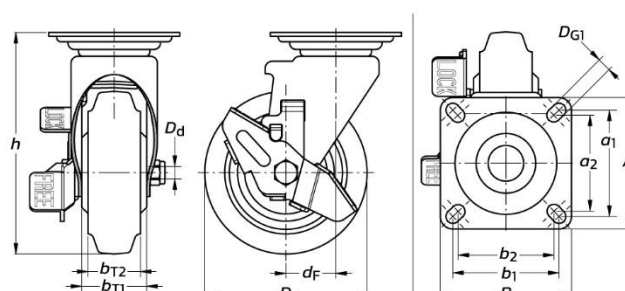
NBJ Swivel Castors (applicable to castor frames with or without wheel brake)
