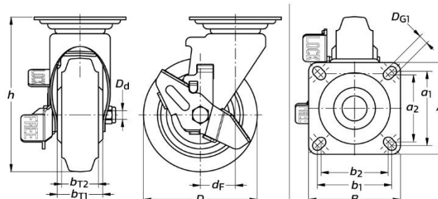
SJ Swivel Castors (applicable to castor frames with or without wheel brake)
