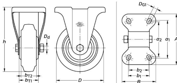
SK Fixed Castors
