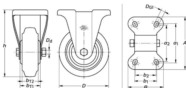
NBK Fixed Castors
