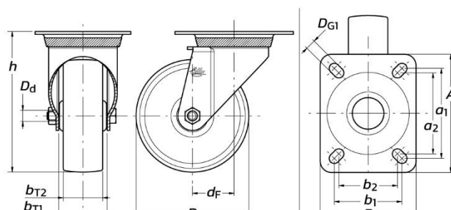
SLJ Swivel Castors
