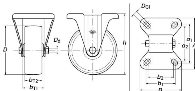
SLK Fixed Castors
